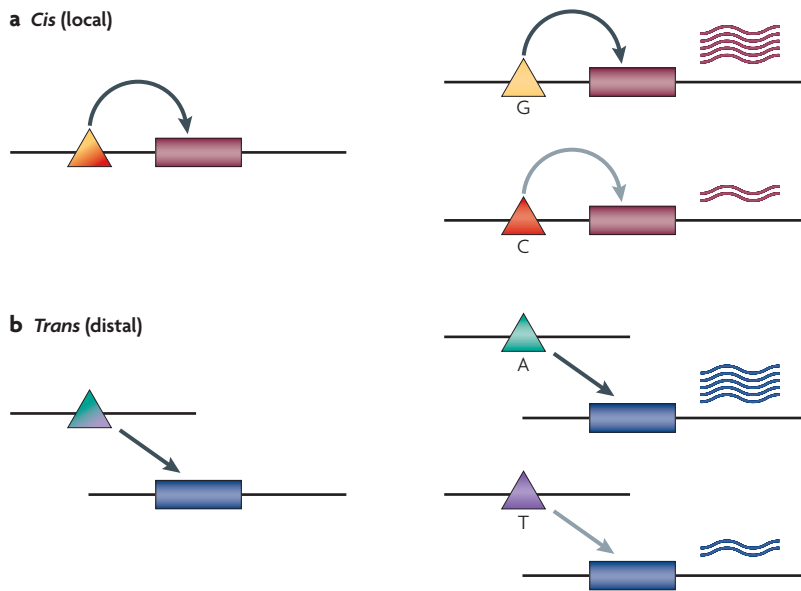
Figure 2 | Effect of cis- and trans-acting DNA variants on expression levels of genes. Polymorphic forms of regulators that act in cis (a) or in trans (b) to the target genes (also called local and distal regulators, respectively) result in variation in expression levels of the target genes. Cis -acting variants are found close to the target genes and trans -acting variants are located far from the target genes, often on another chromosome. Different allelic forms of the cis - and trans -acting variants have different influence on gene expression. In this example, individuals with the G variant of the cis regulator have a higher expression level of the target gene than individuals with the C variant of the regulator. Similarly, individuals with the A variant of the trans regulator have a higher expression level of the target gene than those with the T variant of the regulator.
