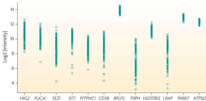
Figure 1 | Inter-individual variation in gene expression levels. Shown are the expression levels of 12 genes in unrelated individuals. Each circle represents the expression level in one individual. The expression levels of two genes, PARK7 and ATP5J2 , are less variable than the other 10 genes, even though the 12 genes were measured using the same cells and methods.
