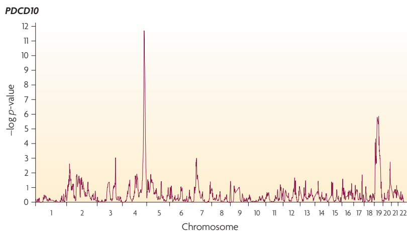
Figure 4 | The expression level of programmed cell death 10 ( PDCD10 ) is trans regulated. PDCD10 is located on chromosome 3. Linkage results show that regulators of this gene are located on chromosomes 4 and 19.
